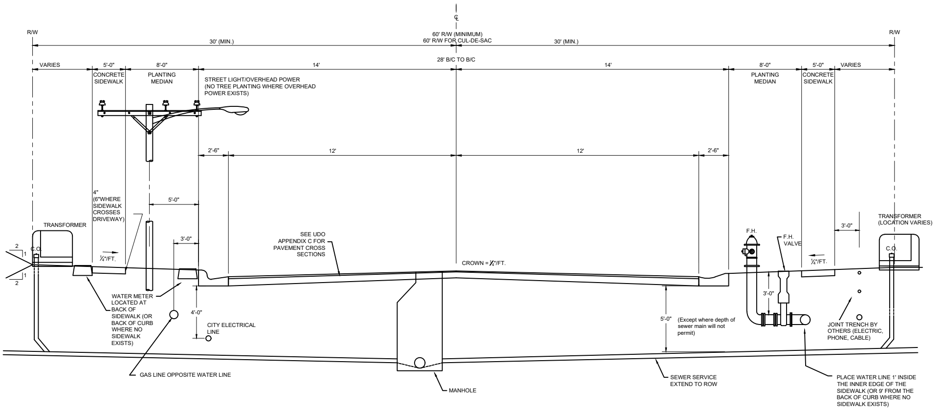
TYPICAL UTILITY LAYOUT NTS
